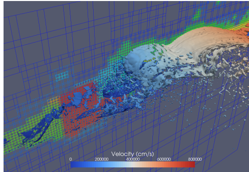
A CTH simulation that generates AMR data. We have used ParaView to visualize CTH simulation AMR data comprising billions of cells, 100's of thousands of blocks, and eleven levels of hierarchy (not shown).
