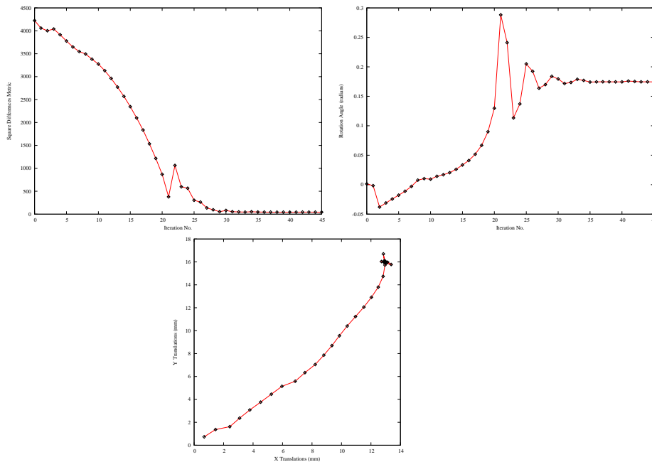
Figure 8.22: Metric values, rotation angle and translations during the registration using the Centered-Rigid2D transform on an image with rotation and translation mis-registration.
