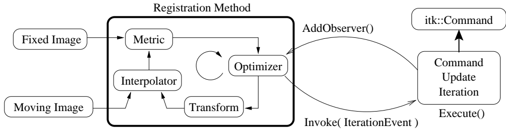
Figure 8.8: Interaction between the Command/Observer and the Registration Method.
