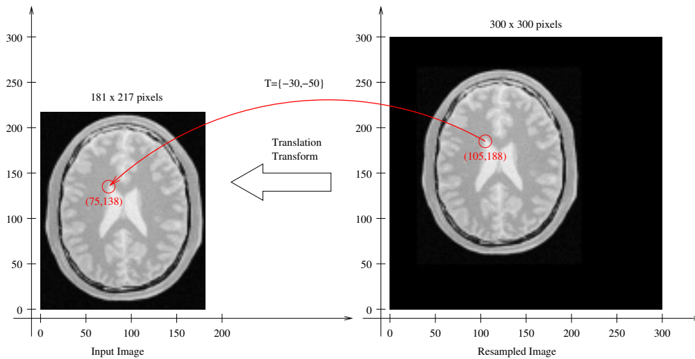
Figure 6.42: ResampleImageFilter. Analysis of a translation by (-30, -50) .
