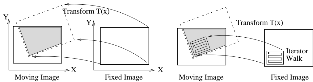
Figure 8.43: The moving image is mapped into the fixed image space under some spatial transformation. An iterator walks through the fixed image and its coordinates are mapped onto the moving image.
