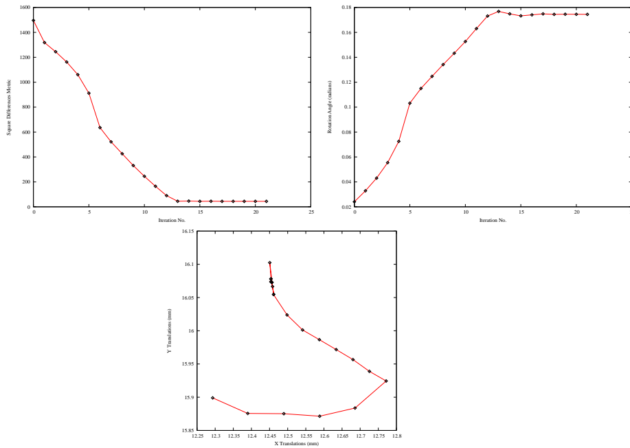
Figure 8.26: Plots of the Metric, rotation angle, center of rotation and translations during the registration using CenteredTransformInitializer .
