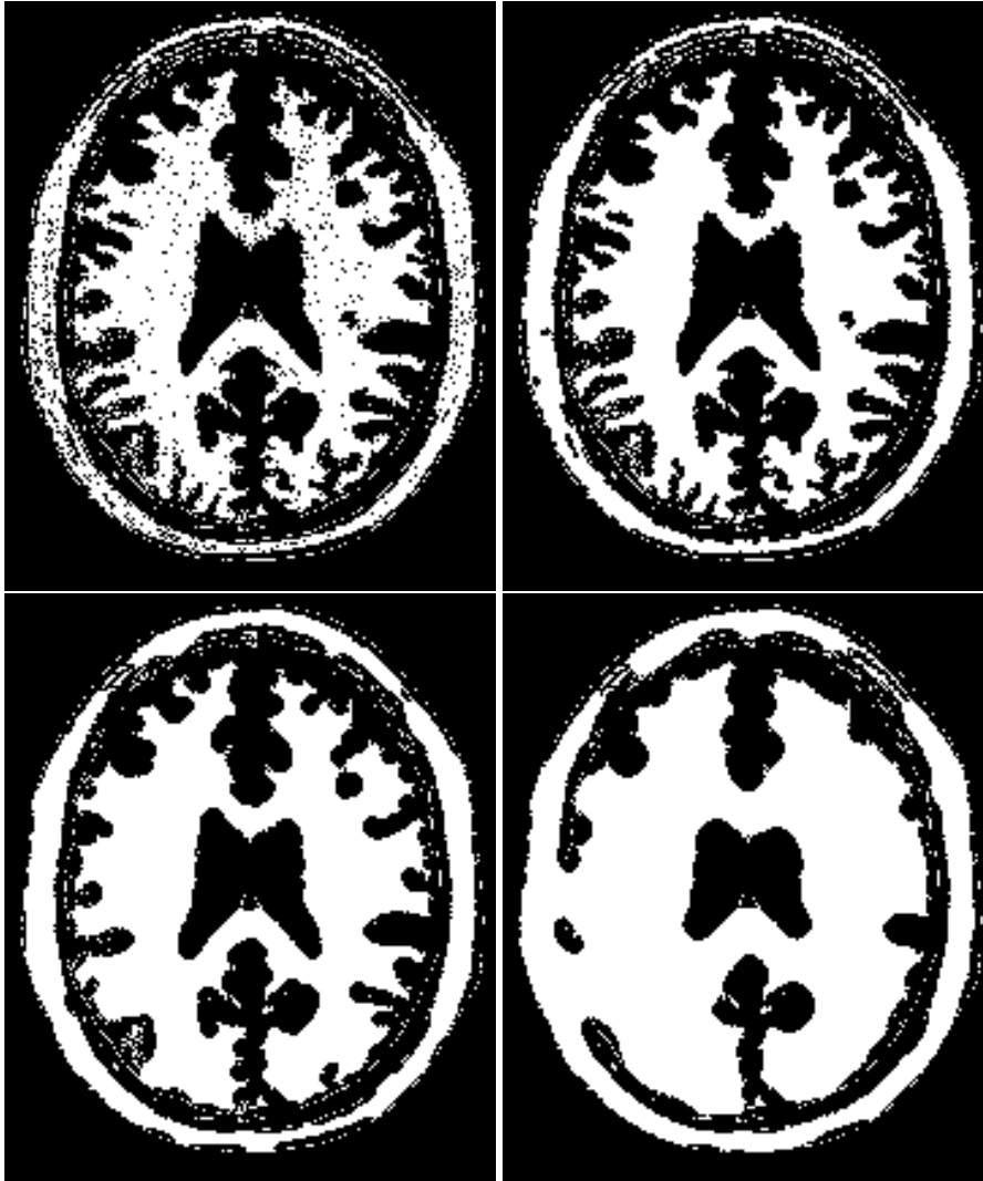
Figure 6.20: Effect of the VotingBinaryIterativeHoleFillingImageFilter on a slice from a MRI proton density brain image that has been thresholded in order to produce a binary image. The output images have used radius 1, 2 and 3 respectively.
