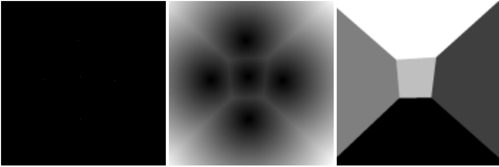
Figure 6.36: DanielssonDistanceMapImageFilter output. Set of pixels, distance map and Voronoi partition.
