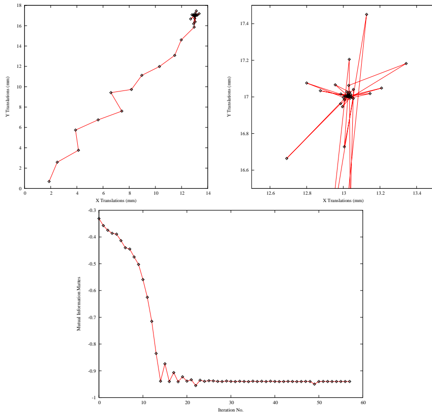
Figure 8.14: Sequence of translations and metric values at each iteration of the optimizer.
