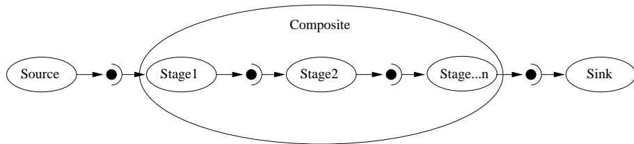
Figure 13.4: A Composite filter encapsulates a number of other filters.
