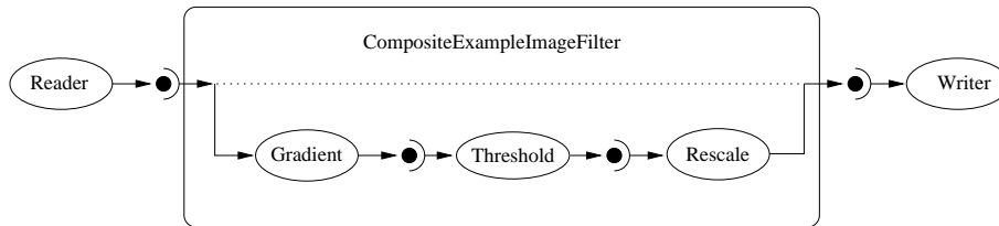
Figure 13.5: Example of a typical composite filter. Note that the output of the last filter in the internal pipeline must be grafted into the output of the composite filter.
