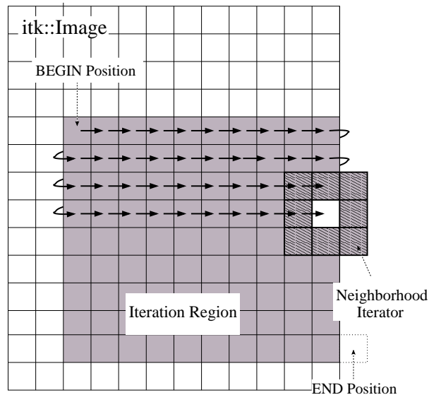
Figure 11.5: Path of a 3 \times 3 neighborhood iterator through a 2D image region. The extent of the neighborhood is indicated by the hashing around the iterator position. Pixels that lie within this extent are accessible through the iterator. An arrow denotes a single iterator step, the result of one ++ operation.
