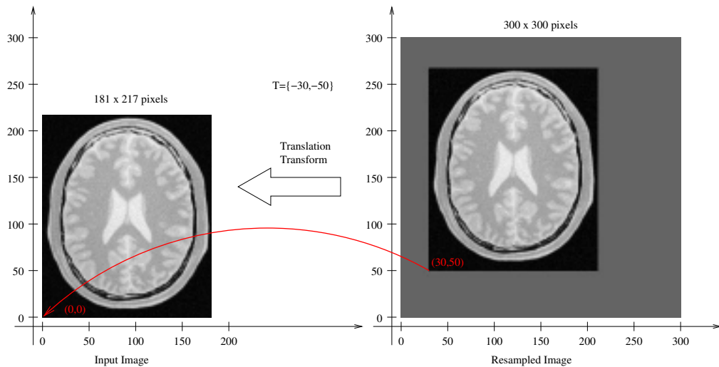
Figure 6.43: ResampleImageFilter highlighting image borders with SetDefaultPixelValue().
