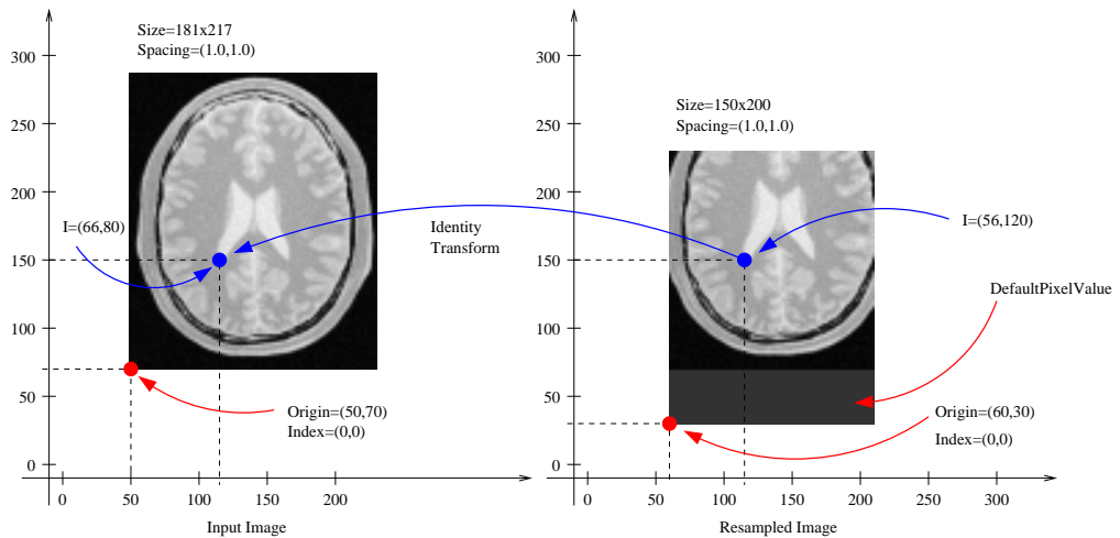
Figure 6.46: Effect of selecting the origin of the input image with ResampleImageFilter.
