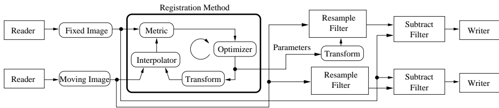
Figure 8.5: Pipeline structure of the registration example.
