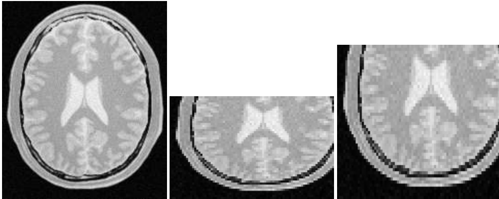
Figure 6.47: Resampling with different spacing seen by a naive viewer (center) and a correct viewer (right), input image (left).
