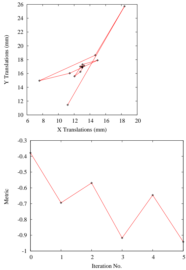
Figure 8.39: Sequence of translations and metric values at each iteration of the optimizer.
