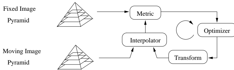
Figure 8.36: Components of the multi-resolution registration framework.
