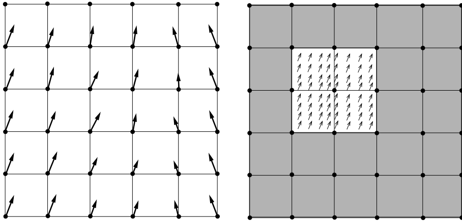
Figure 8.45: The left side illustrates the BSpline grid and the deformations that are known on those nodes. The right side illustrates the region where interpolation is possible when the BSpline is of cubic order. The small arrows represent deformation values that were interpolated from the grid deformations shown on the left side of the diagram.
