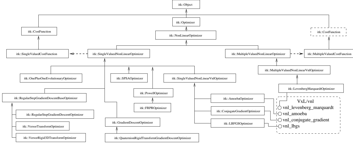
Figure 8.48: Class diagram of the optimizers hierarchy.
