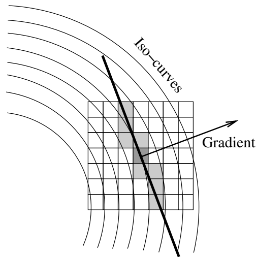
Figure 6.28: Elements involved in the computation of min-max curvature flow.
