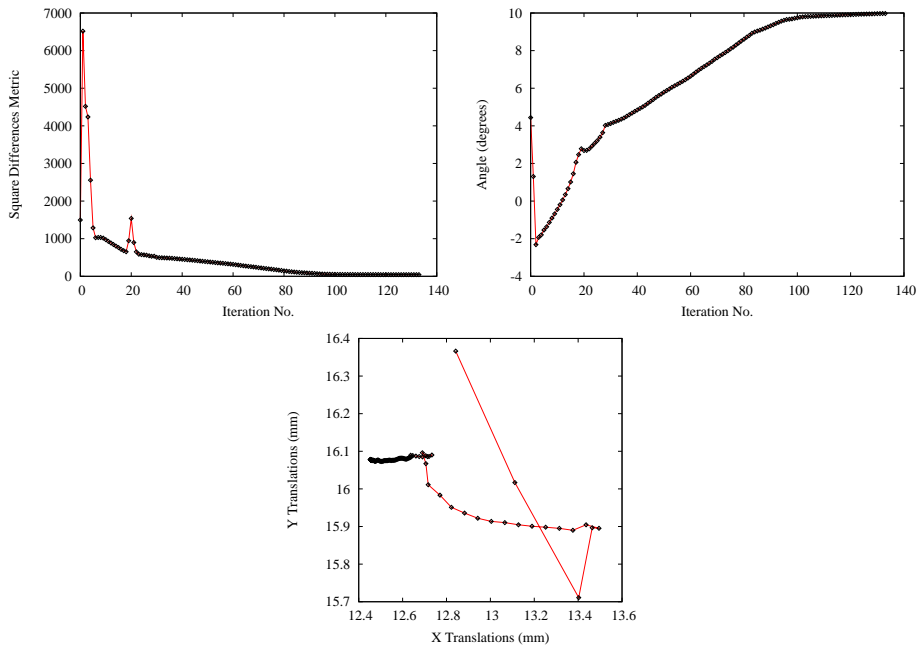
Figure 8.35: Metric values, rotation angle and translations during the registration using the AffineTransform transform.
