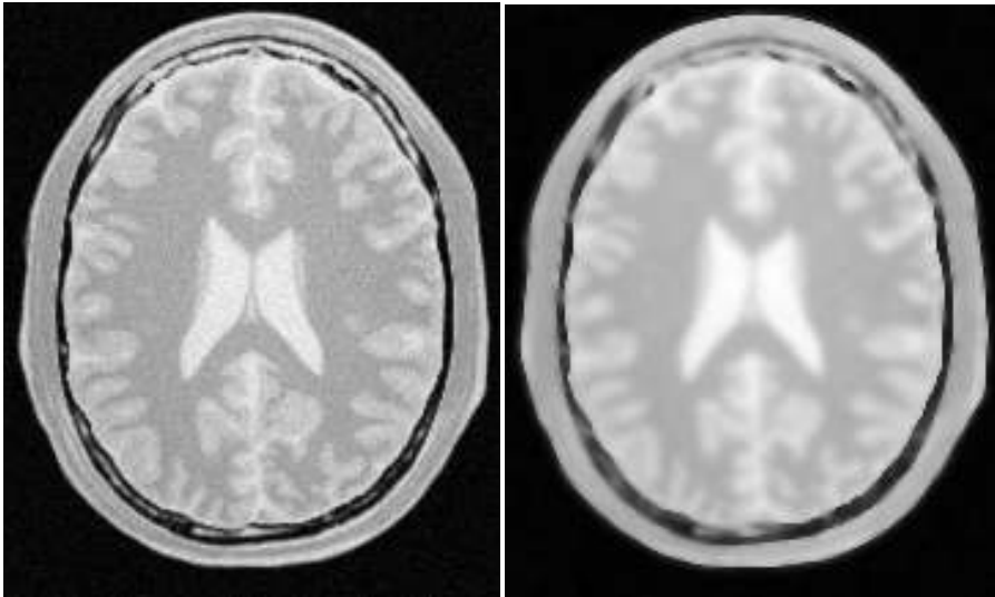
Figure 6.25: Effect of the GradientAnisotropicDiffusionImageFilter on a slice from a MRI Proton Density image of the brain.
