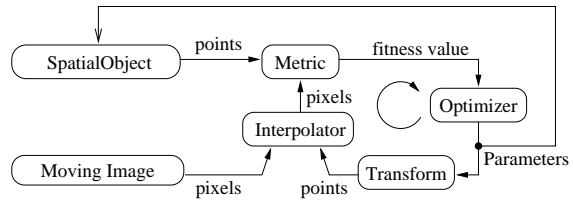
Figure 8.59: The basic components of model based registration are an image, a spatial object, a transform, a metric, an interpolator and an optimizer.
