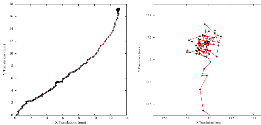
Figure 8.11: Sequence of translations during the registration process. On the left are iterations 0 to 200. On the right are iterations 150 to 200.
