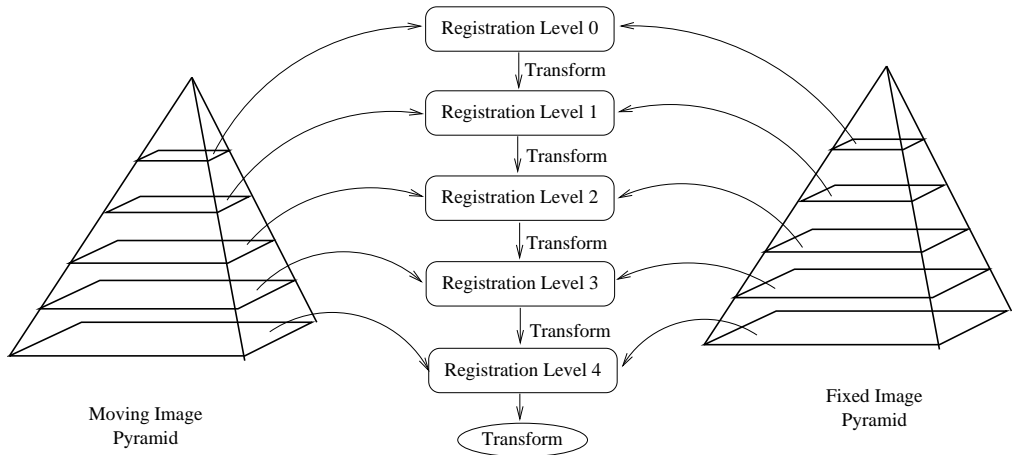
Figure 8.37: Conceptual representation of the multi-resolution registration process.
