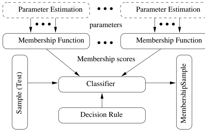
Figure 10.4: Statistical classification framework.
