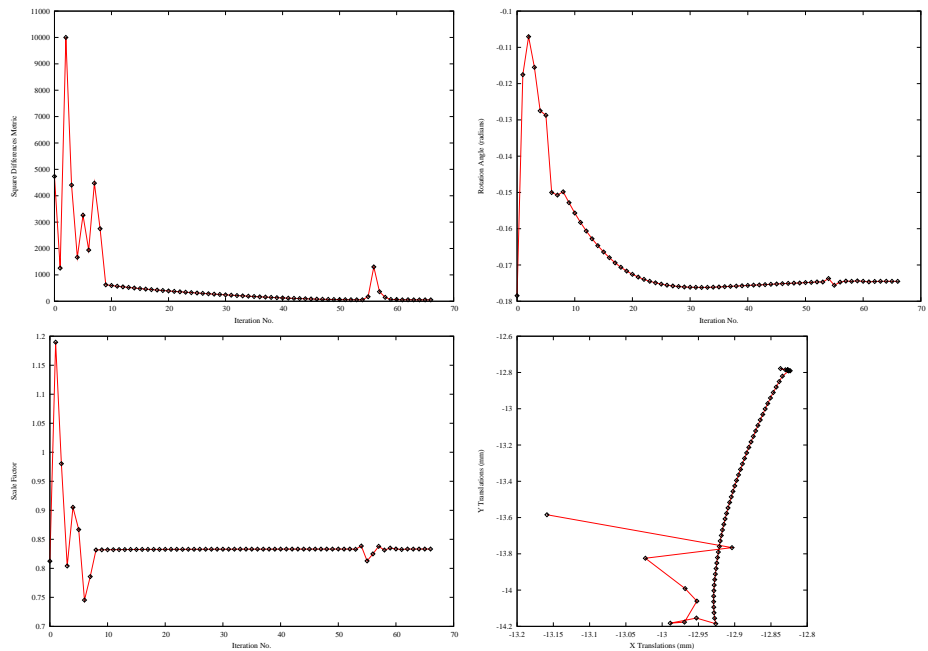
Figure 8.29: Plots of the Metric, rotation angle and translations during the registration using Similarity2D transform.
