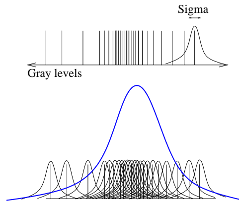
Figure 8.47: In Parzen windowing, a continuous density function is constructed by superimposing kernel functions (Gaussian function in this case) centered on the intensity samples obtained from the image.
