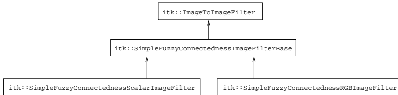
Figure 9.36: Inheritance diagram for the fuzzy connectedness filter.
