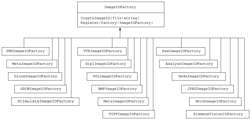
Figure 7.3: Class diagram of the ImageIO factories.
