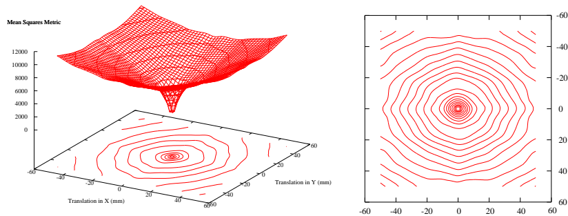
Figure 8.46: Plots of the Mean Squares Metric for an image compared to itself under multiple translations.
