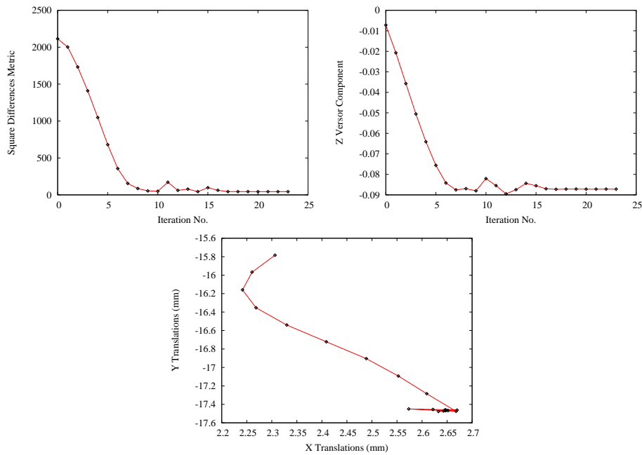
Figure 8.32: Plots of the metric, rotation angle, center of rotation and translations during the registration using CenteredTransformInitializer .
