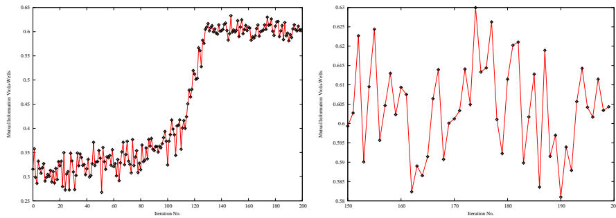
Figure 8.12: The sequence of metric values produced during the registration process. On the left are iterations 0 to 200. On the right are iterations 150 to 200.
