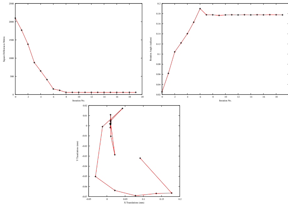
Figure 8.19: Metric values, rotation angle and translations during registration with the CenteredRigid2D transform.
