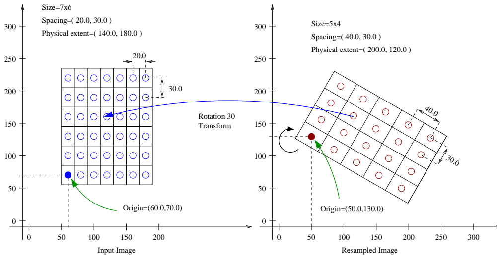
Figure 6.52: Input and output image placed in a common reference system.
