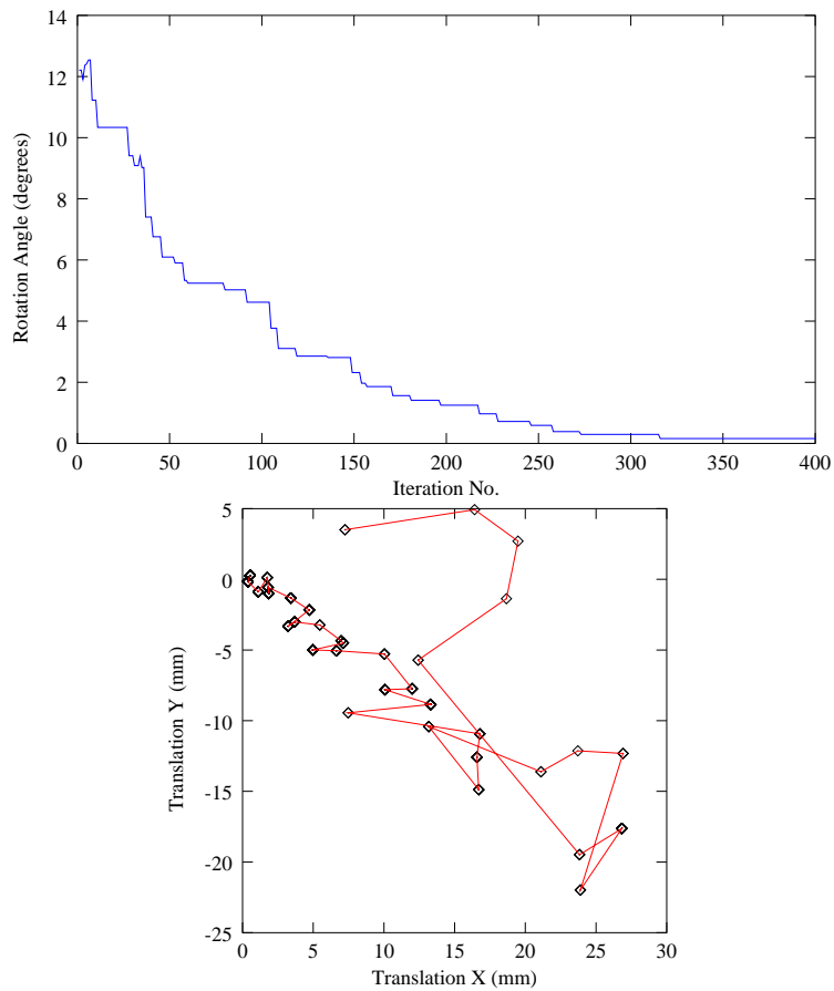
Figure 8.61: Plots of the angle and translation parameters for a registration process between an spatial object and an image.
