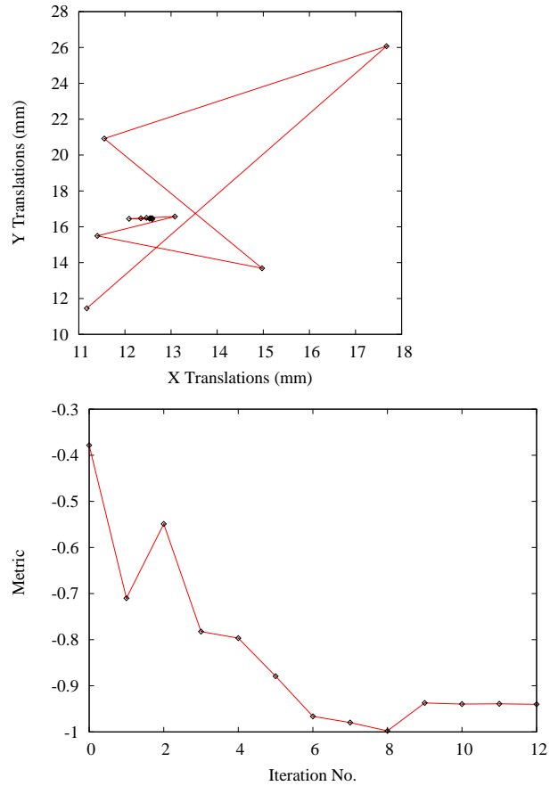
Figure 8.41: Sequence of translations and metric values at each iteration of the optimizer for multi-resolution with the AffineTransform class.
