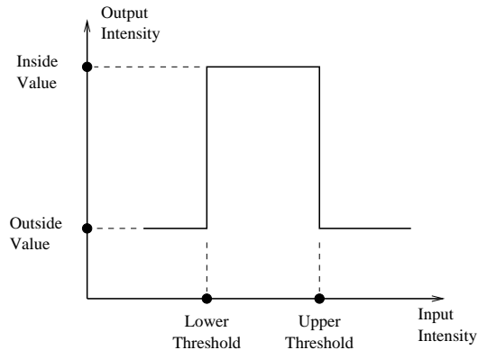
Figure 6.1: Transfer function of the BinaryThresholdImageFilter .
