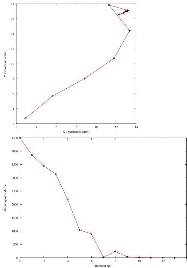
Figure 8.6: The sequence of translations and metric values at each iteration of the optimizer.
