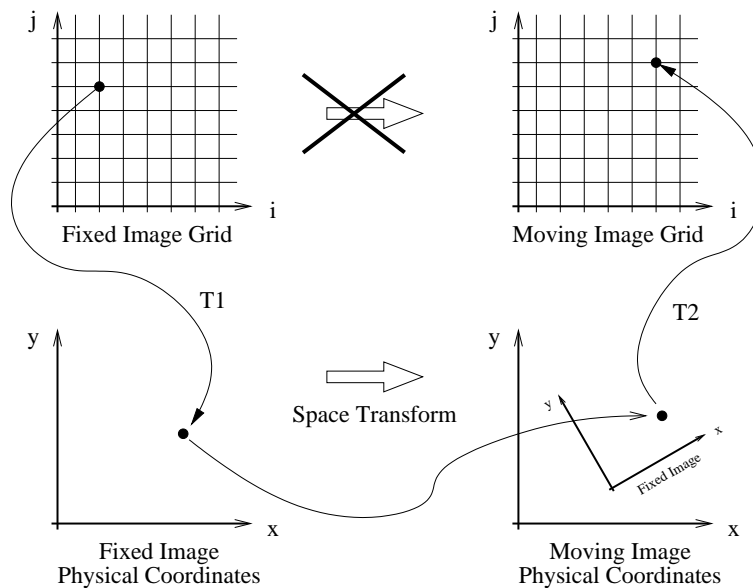
Figure 8.7: Different coordinate systems involved in the image registration process. Note that the transform being optimized is the one mapping from the physical space of the fixed image into the physical space of the moving image.
