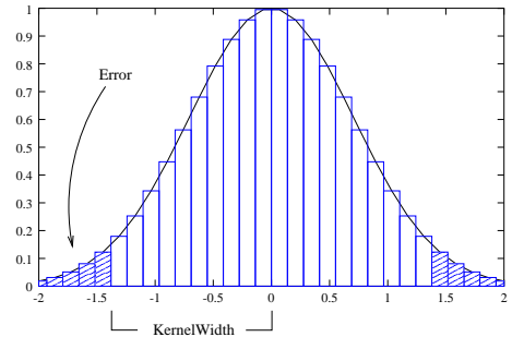
Figure 6.21: Discretized Gaussian.
