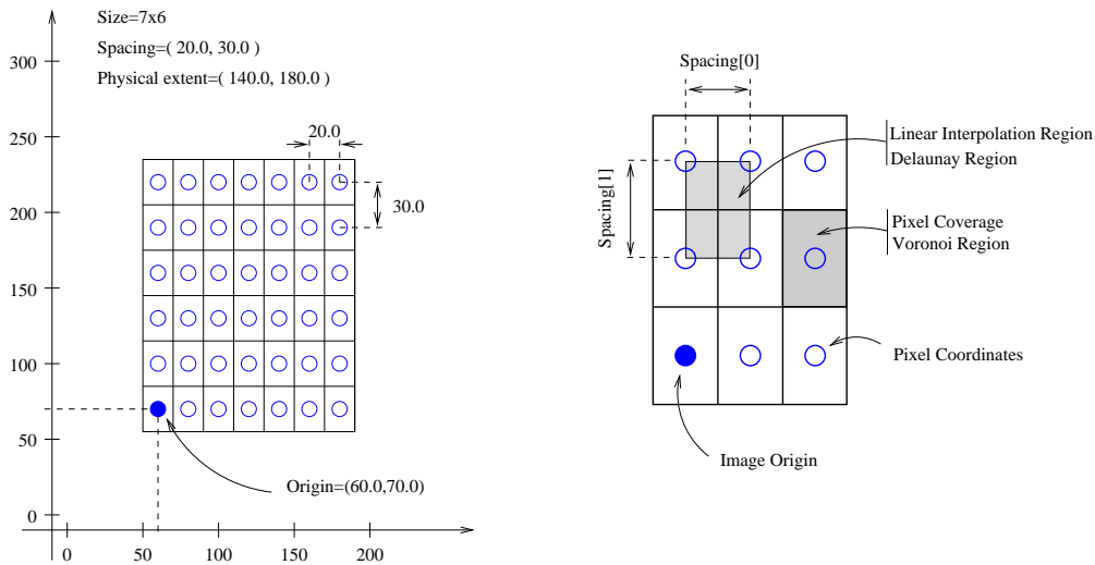
Figure 4.1: Geometrical concepts associated with the ITK image.
