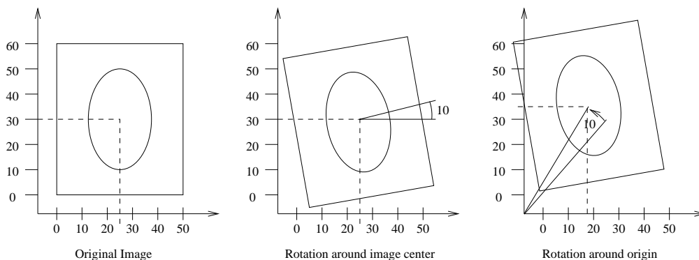
Figure 8.23: Effect of changing the center of rotation.
