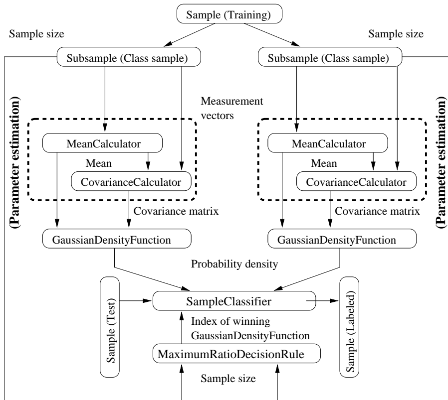
Figure 10.7: Bayesian plug-in classifier for two Gaussian classes.
