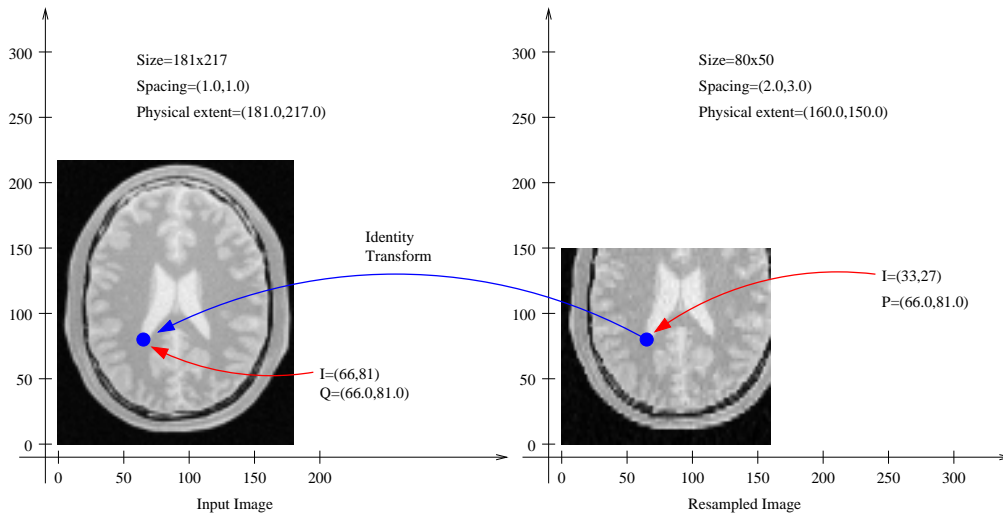
Figure 6.48: Effect of selecting the spacing on the output image.
