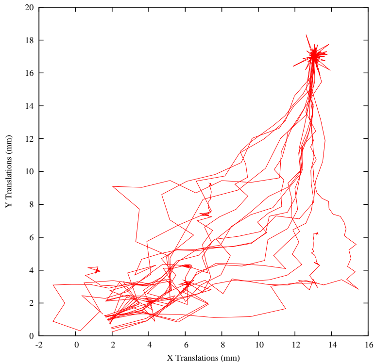
Figure 8.15: Sensitivity of the optimization path to the number of Bins used for estimating the value of Mutual Information with Mattes et al. approach.
