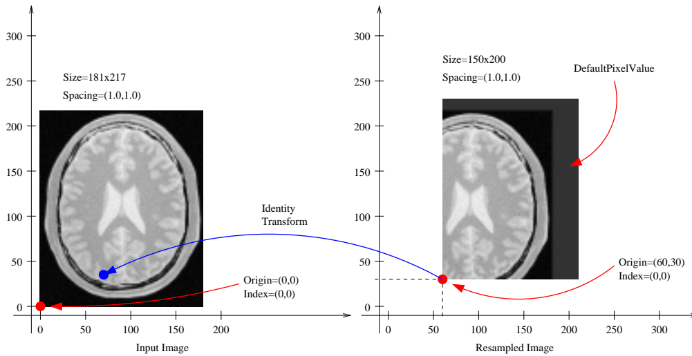
Figure 6.45: ResampleImageFilter selecting the origin of the output image.
